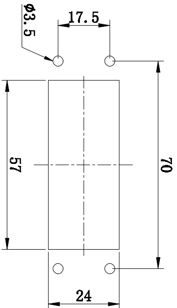
面板开孔图 Panel cut out
