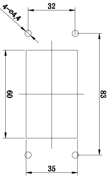
面板开孔图 Panel cut out
