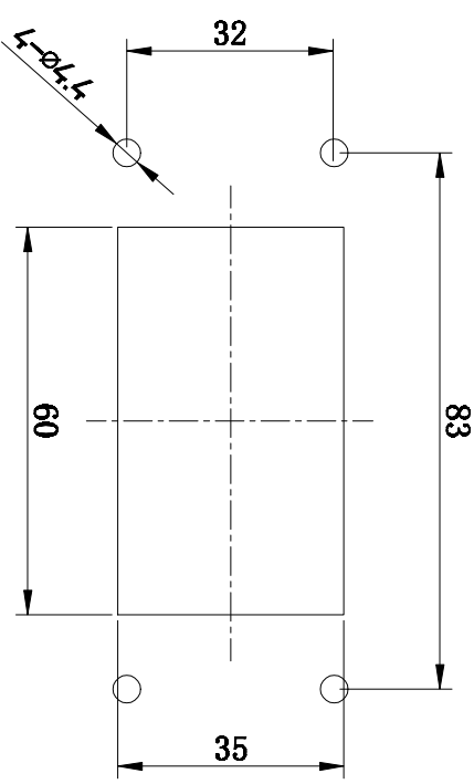
Panel cut out 面板开孔图
