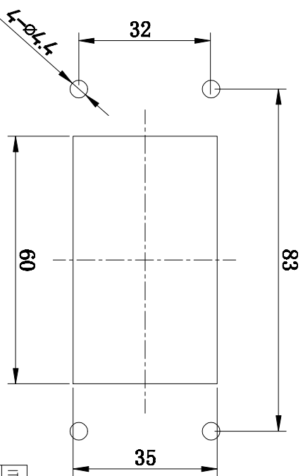
面板开孔图 Panel cut out
