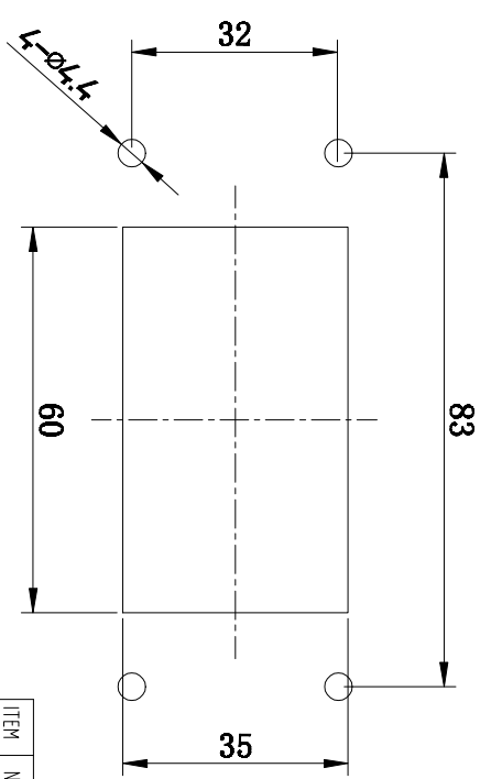
面板开孔图 Panel cut out
