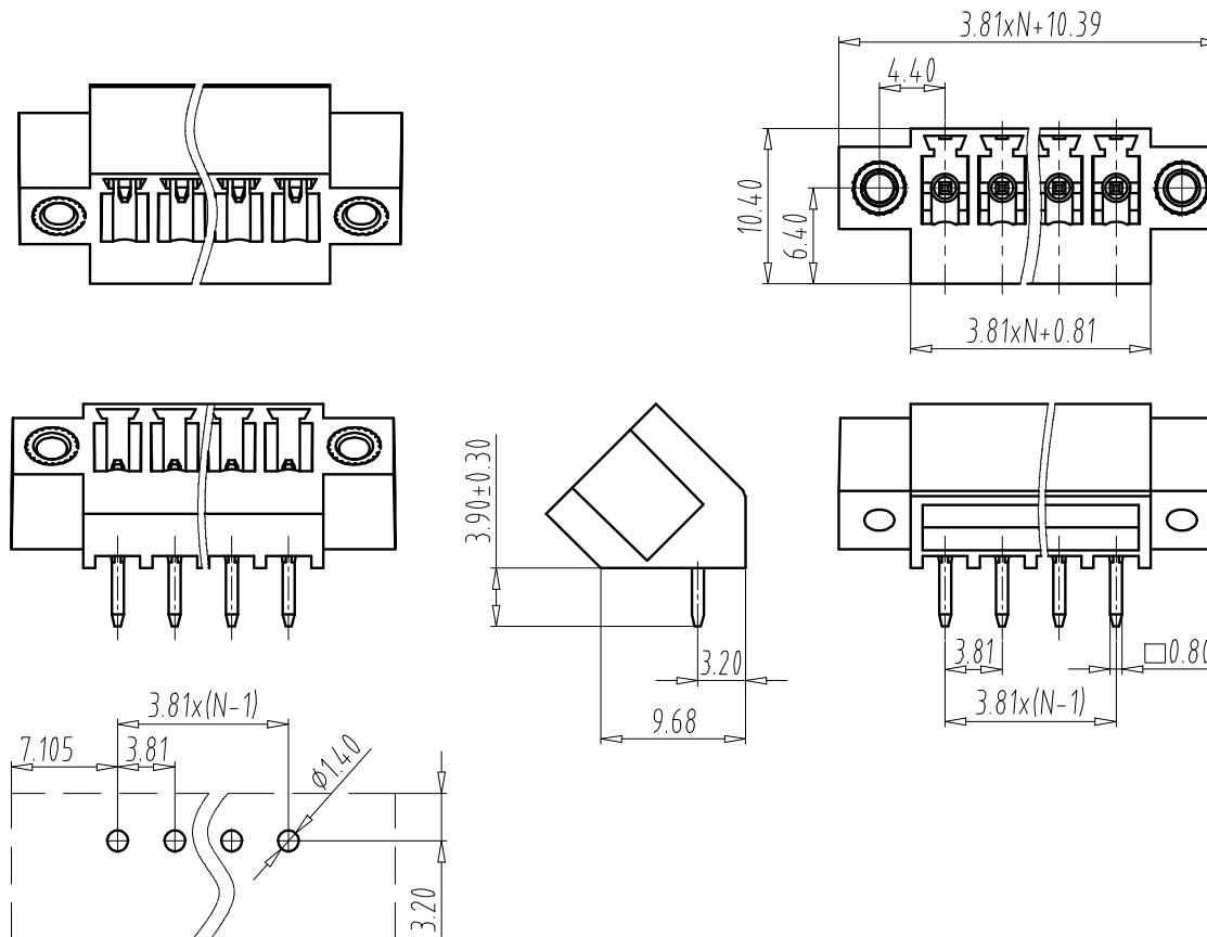
PCB LAYOUT
