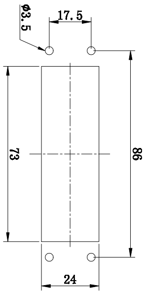
面板开孔图 Panel cut out
