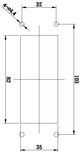
面板开孔图 Panel cut out
