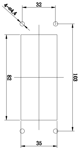
面板开孔图 Panel cut out
