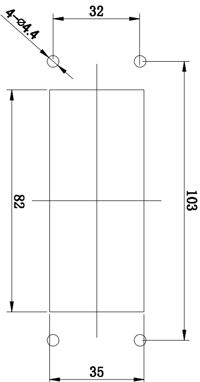
面板开孔图 Panel cut out
