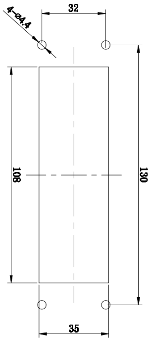
面板开孔图 Panel cut out
