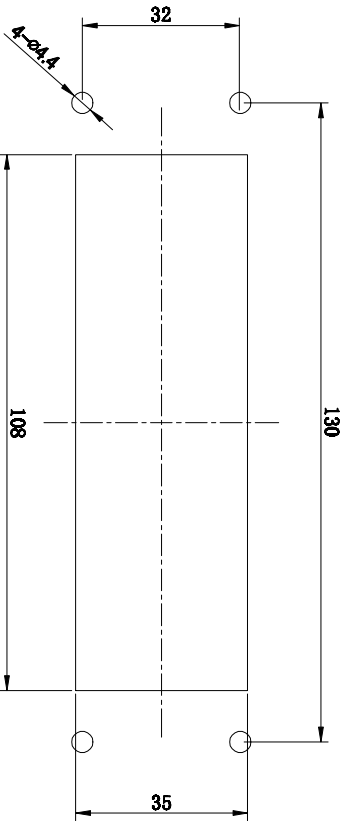
面板开孔图 Panel cut out
