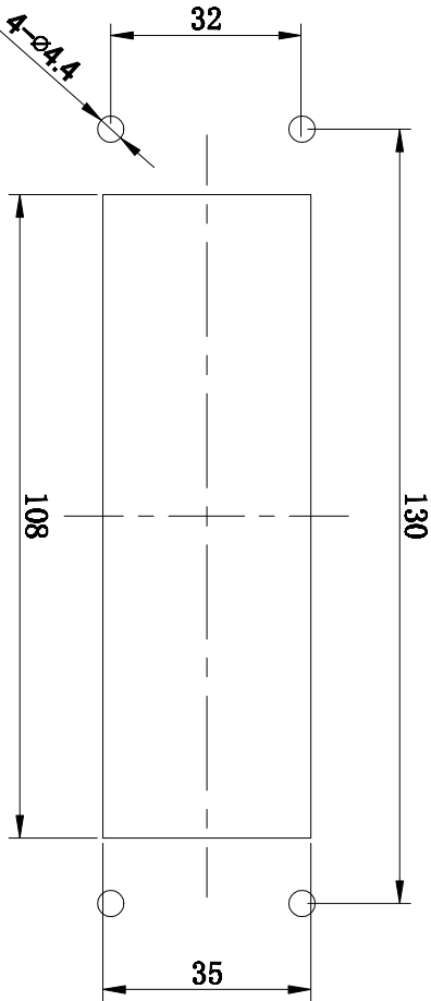
面板开孔图 Panel cut out
