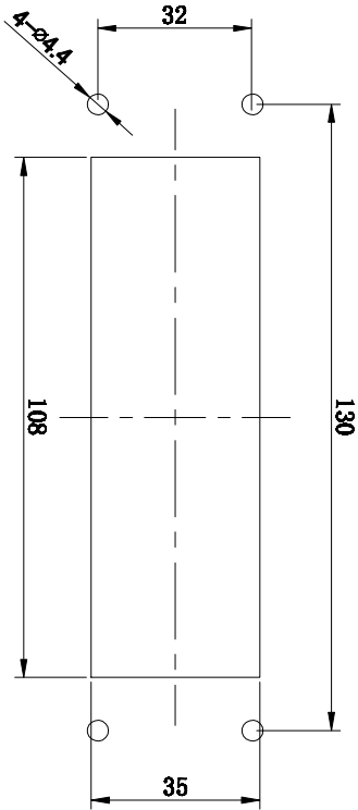
面板开孔图 Panel cut out
