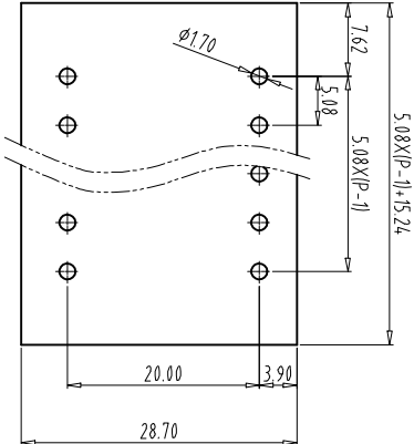
PCB Layout
