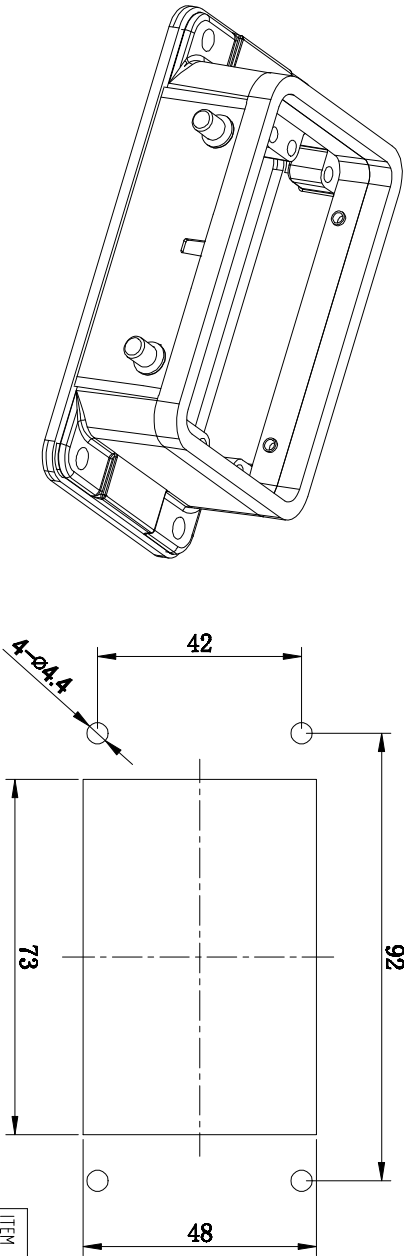
面板开孔图 Panel cut out
