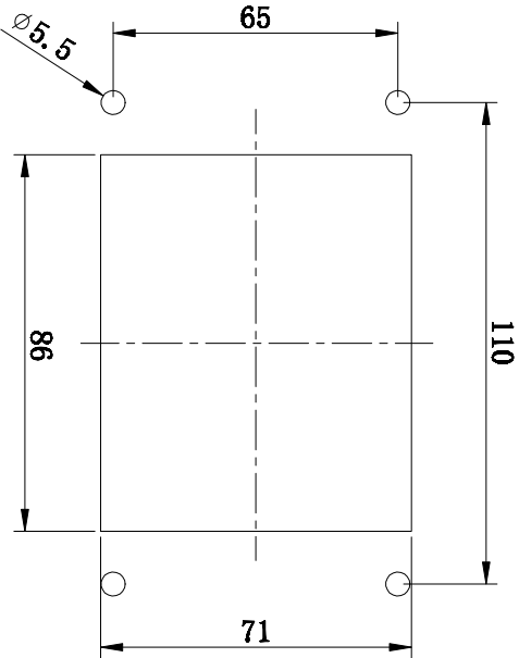
面板开孔图 Panel cut out
