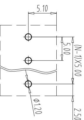
PCB LAYOUT
