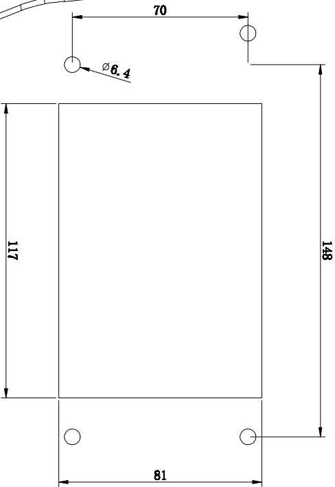
面板开孔图 Panel cut out
