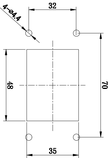
面板开孔图 Panel cut out
