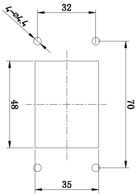
面板开孔图 Panel cut out
