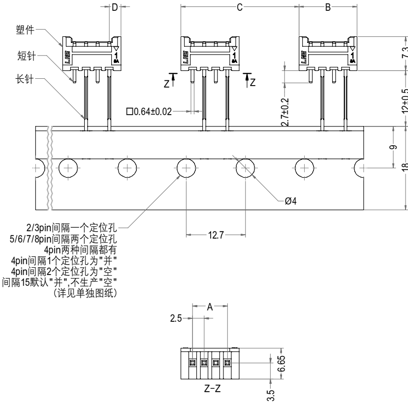
XHQ-4A(1.3长针)编带装(空)
