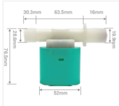
2. 1/2in internal side inlet; green housing
