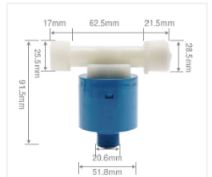
6. 3/4in external side inlet; blue housing
