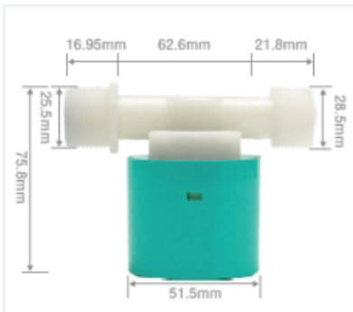
4. 3/4in internal side inlet; green housing
