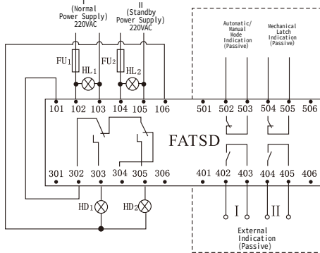
Fully Automatic + Manual (Remote Control) Wiring Mode
