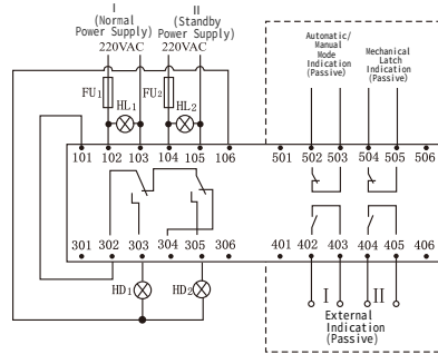
Fully Automatic Wiring Mode
