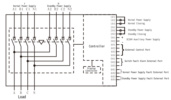
Type F Control 4P Wiring Diagram
