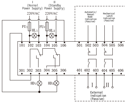
Fully Automatic + Generator Signal Output Wiring Mode
