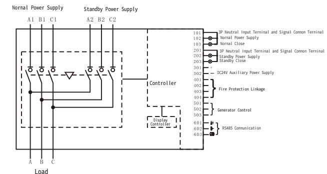
Wiring Diagram for Type A, B, C, D 3-Pole Controllers
