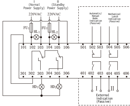
Fully Automatic + Forced “0” (Both Power Supplies Disconnected) Wiring Mode
