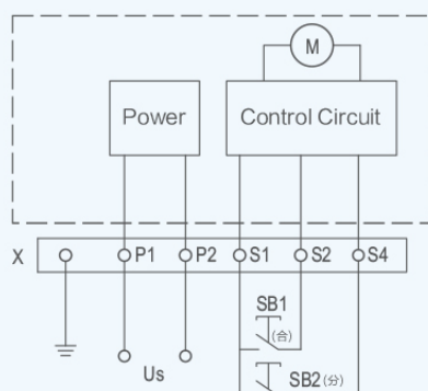
Electric power operator mechanism wiring diagram
