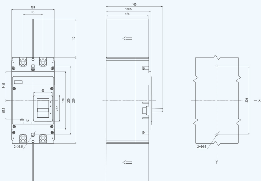
GRM3DC-400/630/800 Outline and installation of hole opening dimensions (2P)
