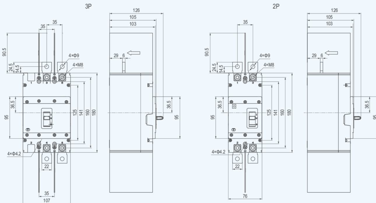
GRM3DC-250/320、GRM3HU-320 Outline and installation of hole opening dimensions
