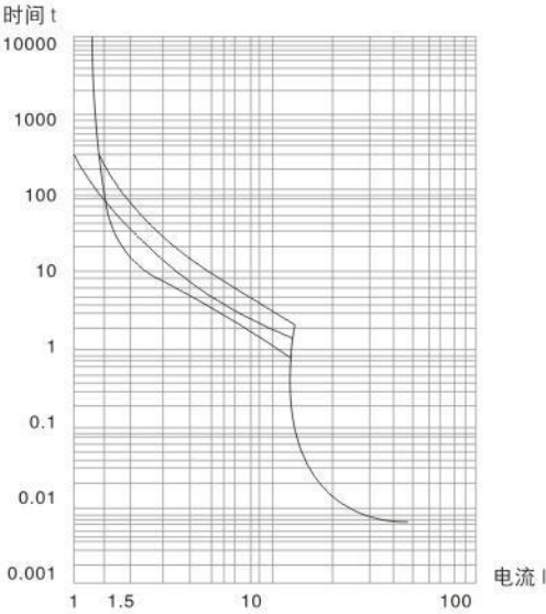
图5 XHV2的热磁脱扣曲线 The hot magnetic disjointing curve of XHV2
