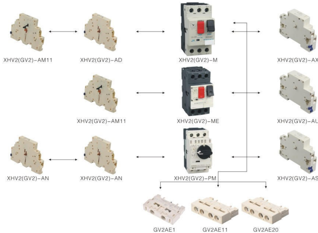
4.1 附加触头 Contacts of accessories
