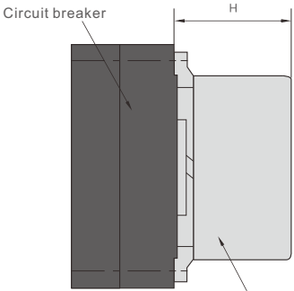
Electrical operation mechanism
