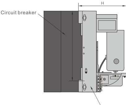
Electrical operation mechanism
