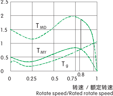
转矩 / 额定转矩 Torque/Rated torque
