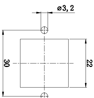
面板开孔图 panel cut out
