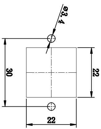
面板开孔图 Panel cut out
