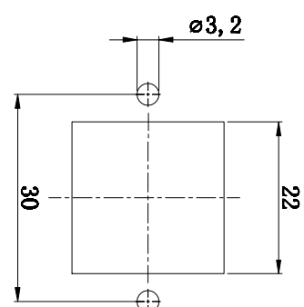
面板开孔图 panel cut out
