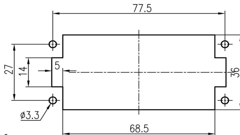
面板安装开孔图 Panel cut out
