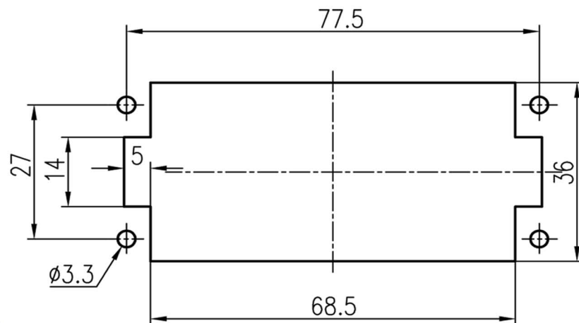
面板安装开孔图 Panel cut out
