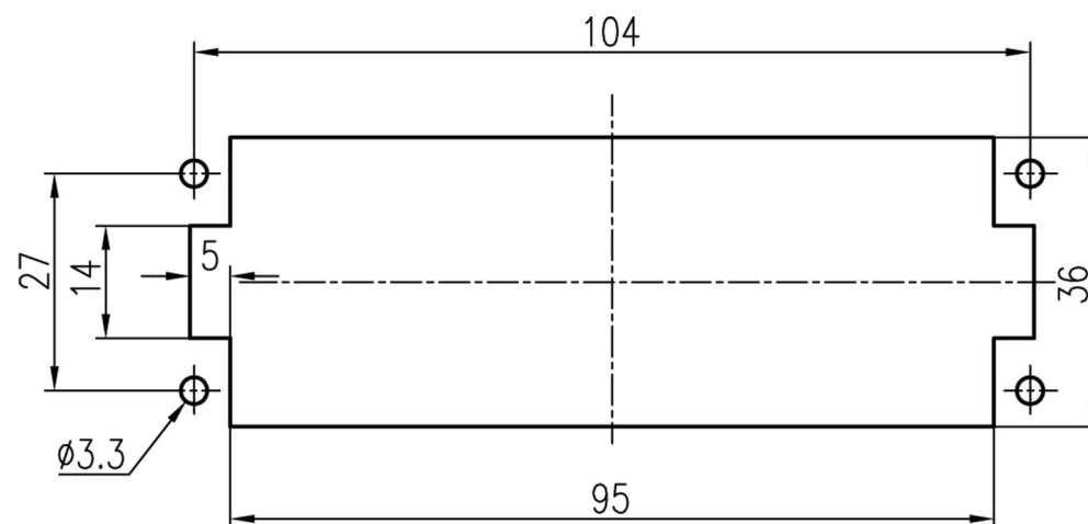
面板安装开孔图 Panel cut out
