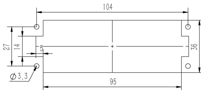
面板安装开孔图 Panel cut out
