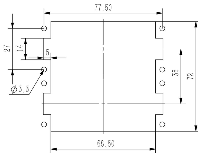
面板安装开孔图 Panel cut out
