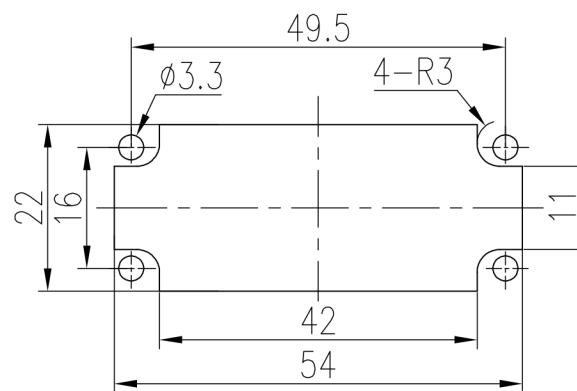
面板安装开孔图 Opening diagram of panel installation
