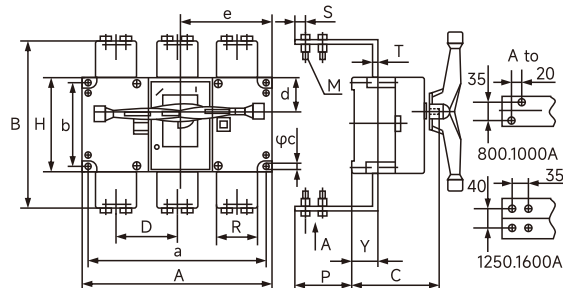
Fig.12, HGL-800~1600A/B behind board wiring disconnect switch 7. Dimensions of HGLC series side-operated disconnecting switches (see Table 8-9 and Figs. 13-16)
