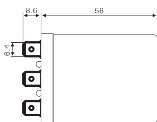
Dimension Drawing of Bottom (Type A) Flange Type
