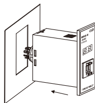
(9) Insert the relay into the panel.
