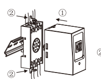
(7) Mount the relay and close the hooks.
