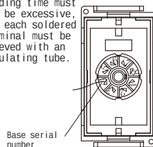
(11) Solder wires according to the base serial number.
