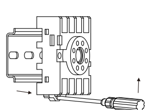
(12) Rail - mounting removal: Pry open the rail clip and remove the base.
