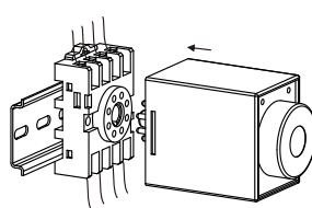
(9) Rail - mounting installation: Install the relay, aligning the protrusions on the relay with the grooves on the base.
