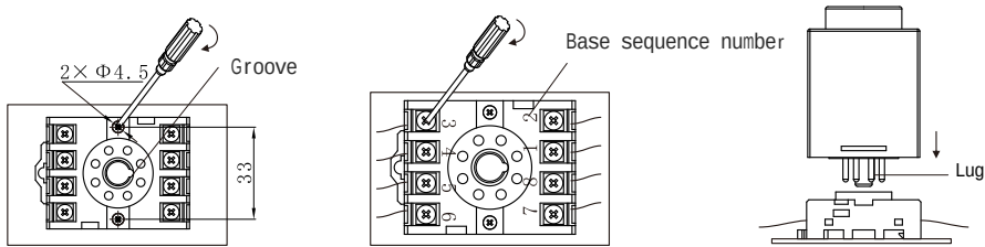
(1) Panel - mounting installation: Tighten the mounting screws.
