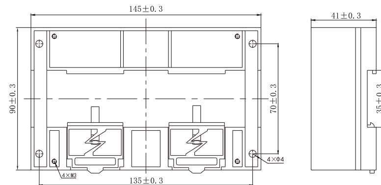
Fixed Hole Mounting and 35mm Guide Rail Mounting
