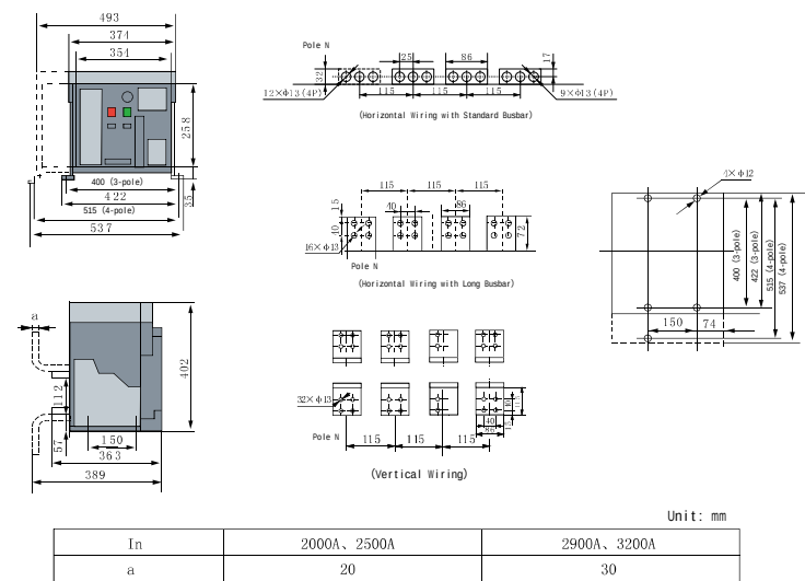
Figure 9 Installation and Outline Dimensions of Fixed Circuit Breaker (XLDW1-3200, 3200/4)
