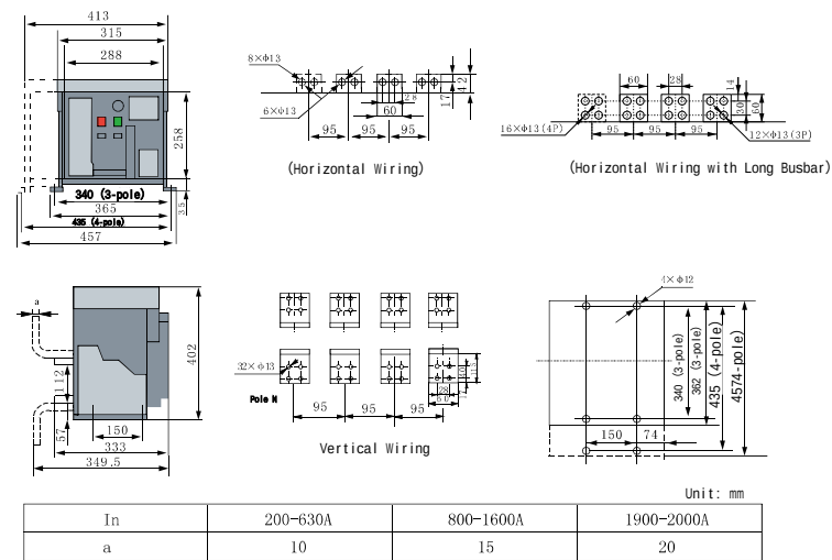
Figure 8 Installation and Outline Dimensions of Fixed Circuit Breaker (XLDW1-2000, 2000/4)
