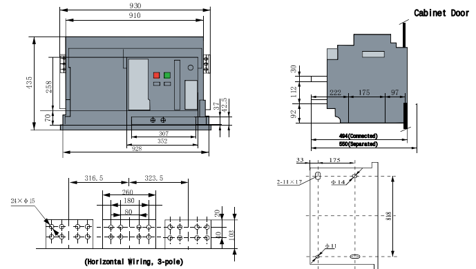
Figure 14 Installation Dimensions and Outline Dimensions of Drawer-Type Circuit Breaker (XLDW1-6300, 6300/4 In=4000A, 5000A)
