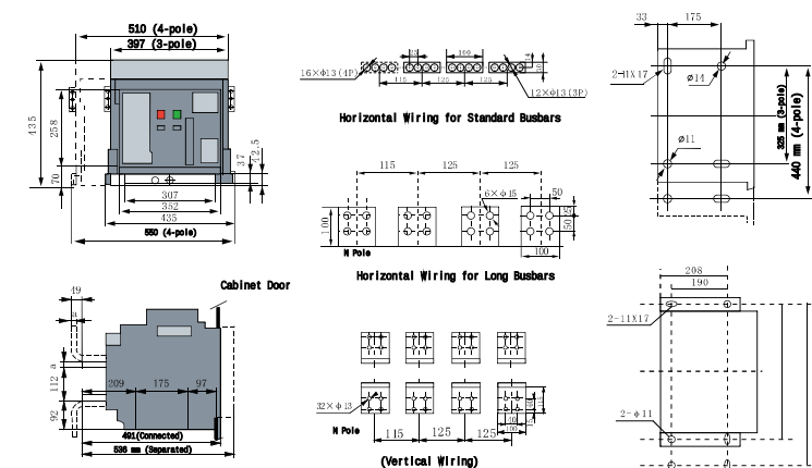
Figure 10 Installation Dimensions and Outline Dimensions of Drawer-Type Circuit Breaker (XLDW1-2000, 2000/4)
