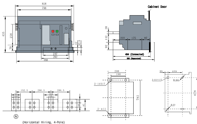
Figure 13 Installation and Outline Dimensions of Drawer-Type Circuit Breaker (XLDWL-4000/4)
