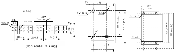
Figure 14 Installation Dimensions and Outline Dimensions of Drawer-Type Circuit Breaker (XLDW1-6300, 6300/4 In=4000A, 5000A)
