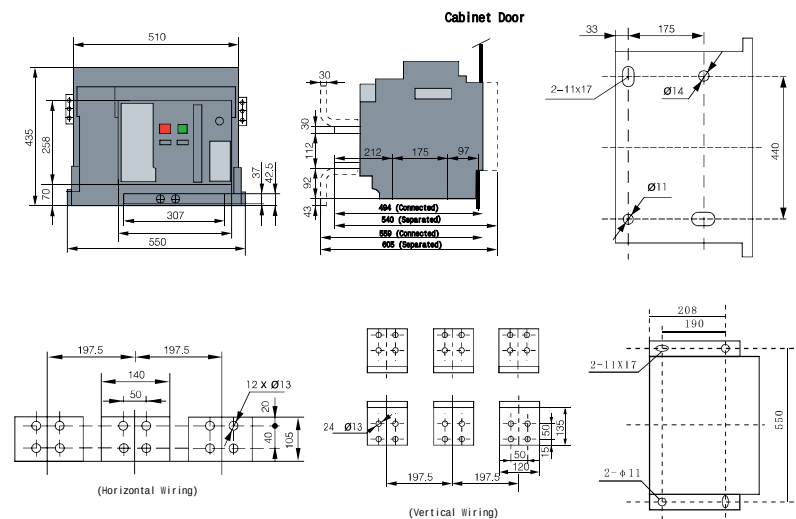
Figure 12 Installation and Outline Dimensions of Drawer-Type Circuit Breaker (XLDWL-4000)
