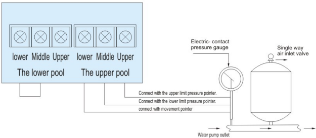
D、Constant pressure connection
