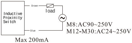
4.AC 2 - Wire Type (Normally Open/Closed)
