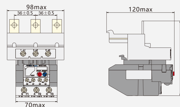
LR2-150/D(with NC7 type) Appearance and Installation
