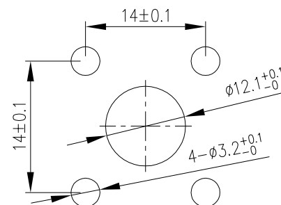
Panel cut
