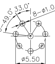
PCB layout
