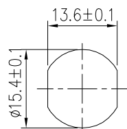
PG9 Panel cut
