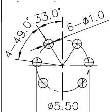
PCB layout
