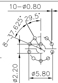
PCB layout
